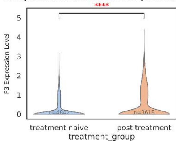
A F3 Expression: treatment naive vs post treatment
